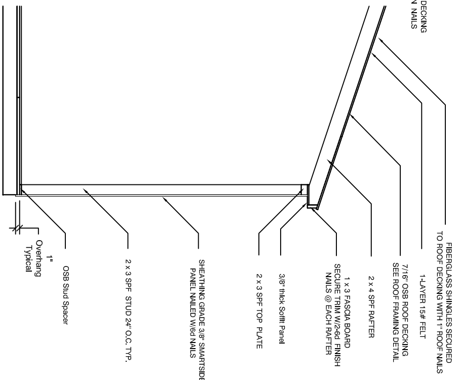
(B) 2 WALL SECTION SCALE: 1/2" = 1'-0"
